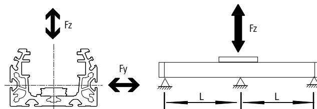
Force F_z
